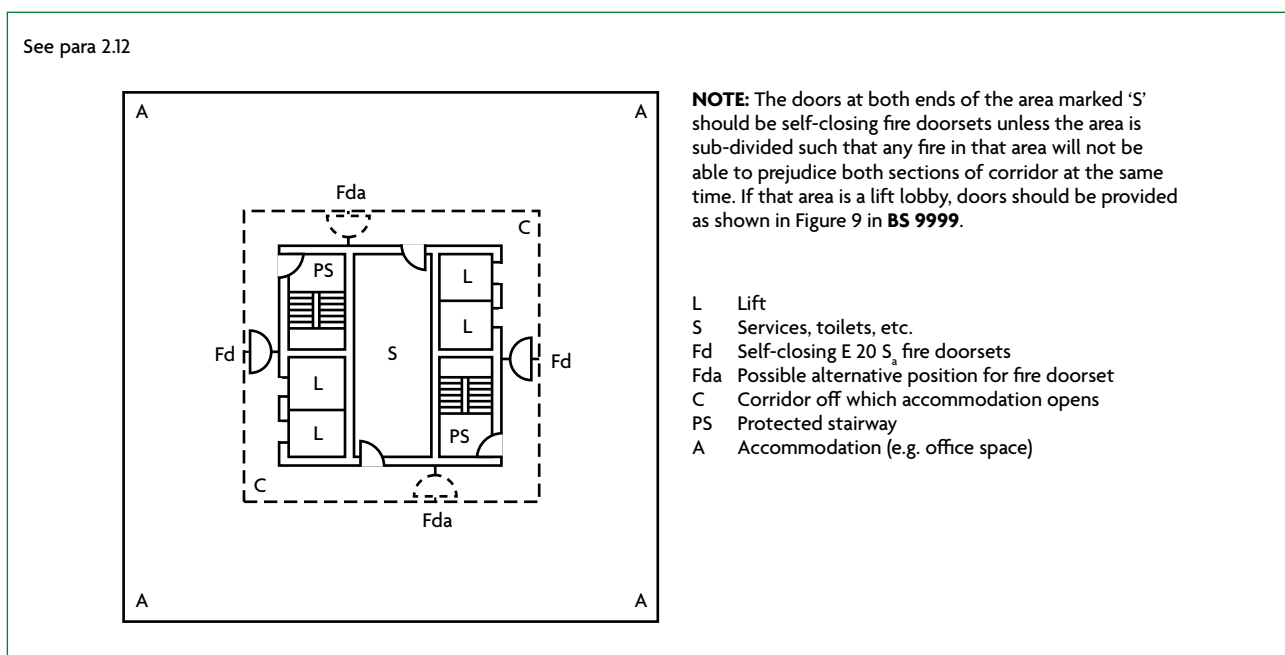
Diagram 2.4 Exits in a central core
